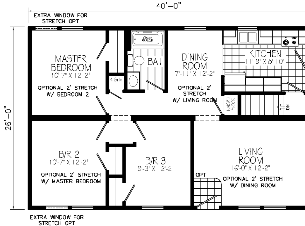
MW401A 26X40 APPROX. 1040 Sq. Ft. NOT AVAILABLE WITH RAISED RANCH OPTION
