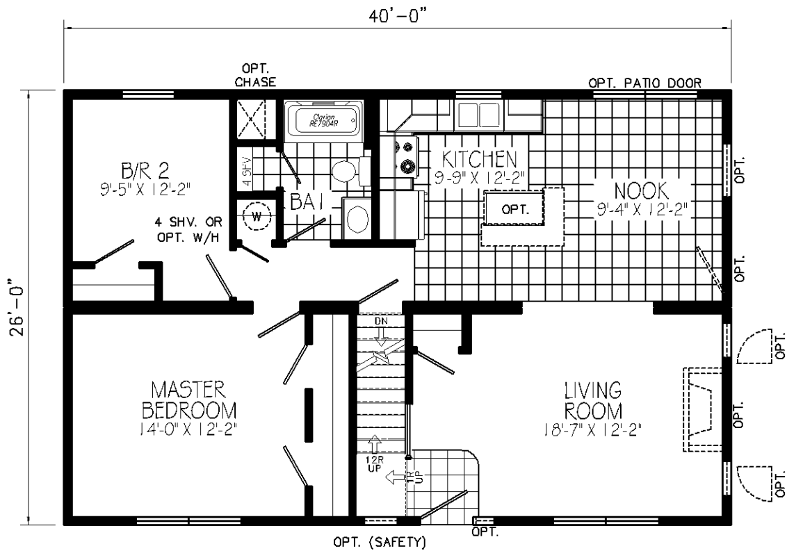
CT002A 26x40 APPROX. 1040 Sq. Ft. NOT AVAILABLE WITH COMPLETE HOUSE PACKAGE
