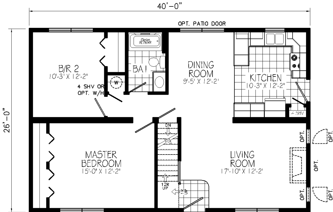
CT015A 26x40 APPROX. 1040 Sq. FT. NOT AVAILABLE WITH COMPLETE HOUSE PACKAGE
