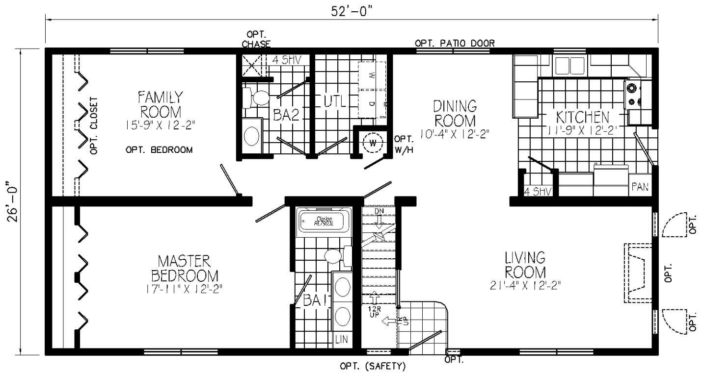
CT008A 26x52 APPROX. 1352 Sq. FT. NOT AVAILABLE W/ COMPLETE HOUSE PACKAGE
