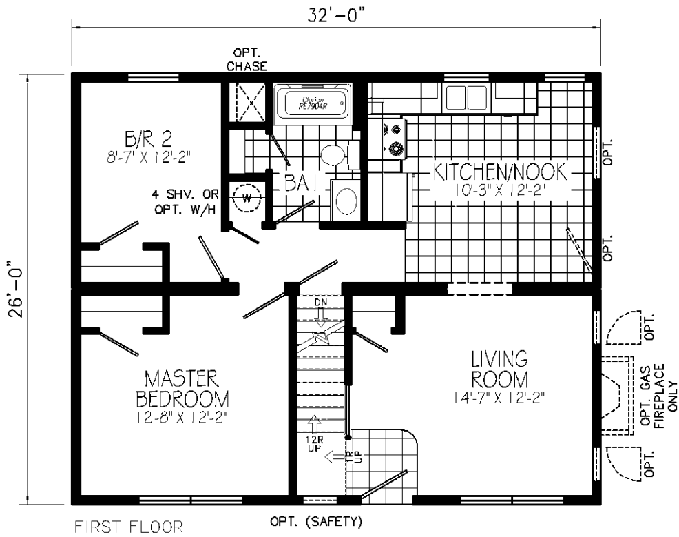
NT403A 26x32 APPROX. 832 Sq. Ft.
