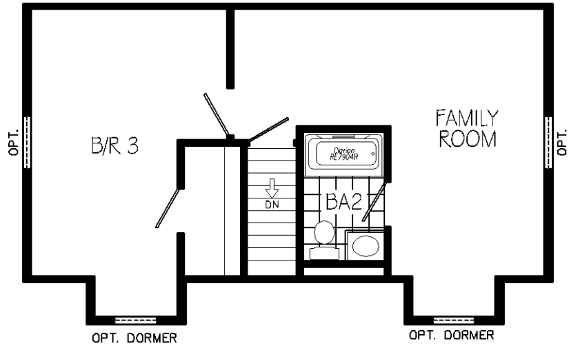
SECOND FLOOR BY OTHERS APPROX. 515 Sq. Ft. UNFINISHED
